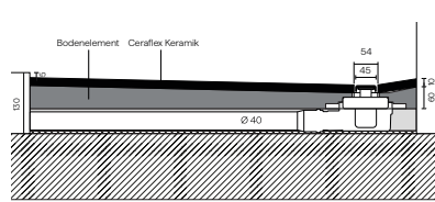
MINIMAX DN 40
